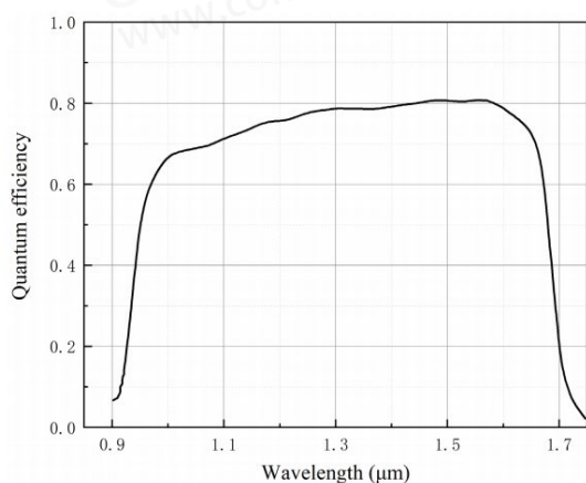
QE Curve
