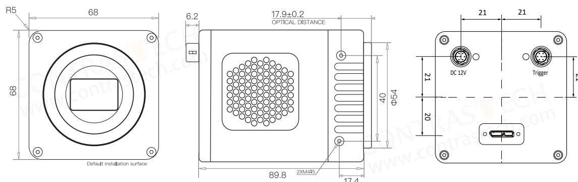
Dimensions A
