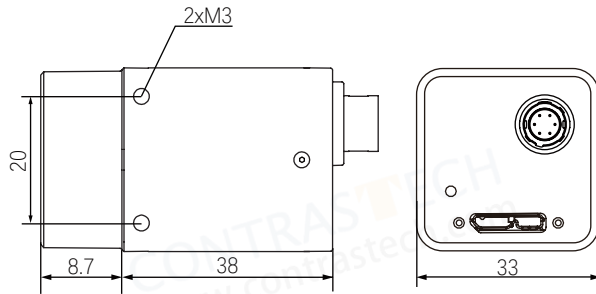
Dimensions E
